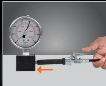
Convenient Engagement To engage the coupler, simply press the thumb lever & slide the coupler onto the fitting. The hardened 6 cylindrical pins hold the grease/zerk fitting tight.
